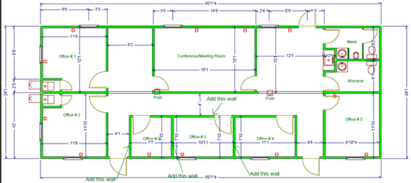
24' x 60' Frameless Wet Office Complex (CPX 81763)
