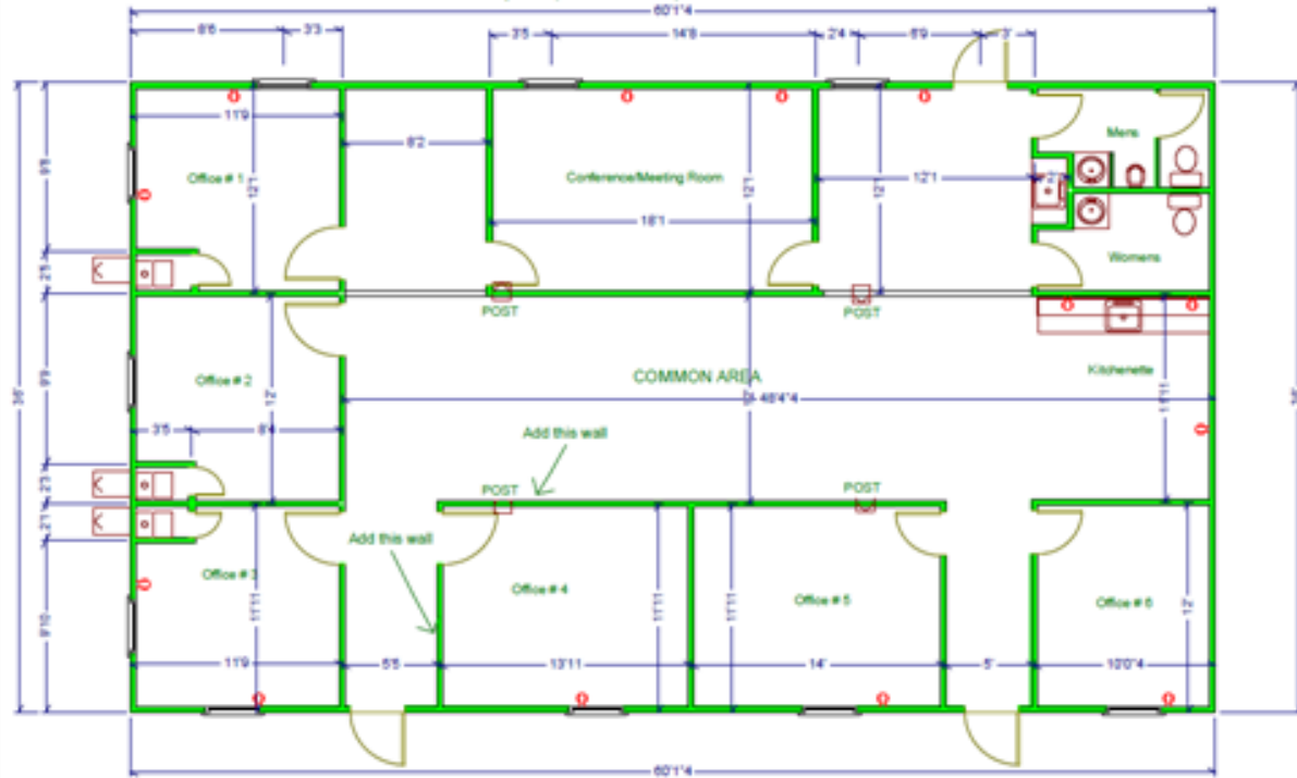
36' x 60' Frameless Wet Office Complex (CPX 81763)
